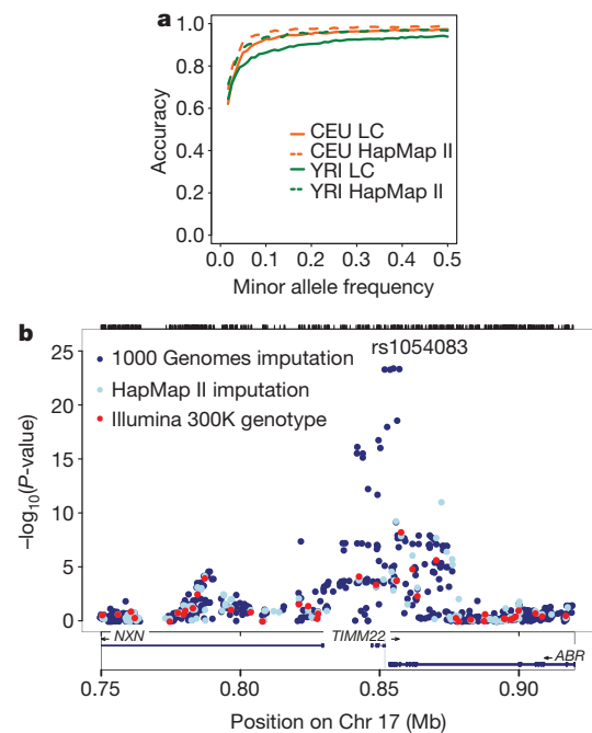
Figure 4 | Imputation from the low-coverage data. a , Accuracy of imputing variant genotypes using HapMap 3 sites to impute sites from the low-coverage (LC) project into the trio fathers as a function of allele frequency. Accuracy of imputing genotypes from the HapMap II reference panels 4 is also shown. Imputation accuracy for common variants was generally a few per cent worse from the low-coverage project than from HapMap, although error rates increase for less common variants. b , An example of imputation in a cis-eQTL for TIMM22 , for which the original Illumina 300K genotype data gave a weak signal 28 . Imputation using HapMap data made a small improvement, and imputation using low-coverage haplotypes provided a much stronger signal.
